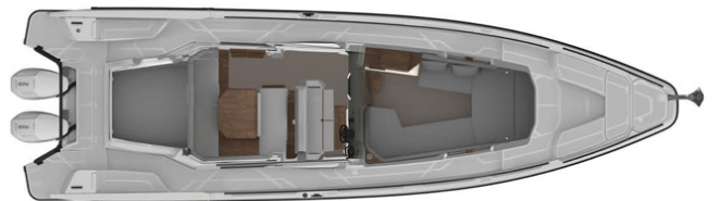
Standard sofa layout and driver's sofa with flip-up bolsters and reversable backrest. Bar cabinet on portside wall.
